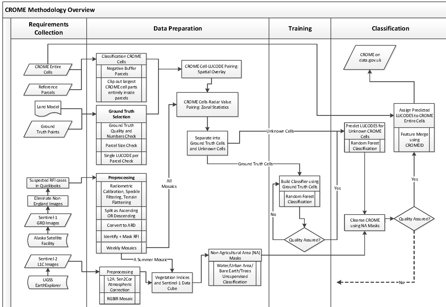
Figure 3. Workflow for CROME classification
